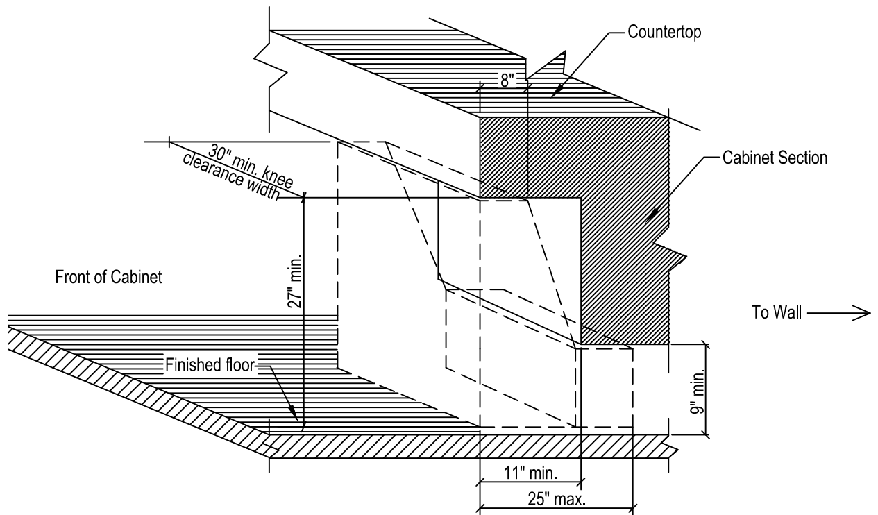
Knee Clearance
